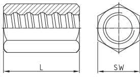
tuerca hexagonal larga EP anchor nut EP long
