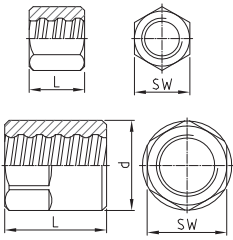
contratuercas larga lock nut long
